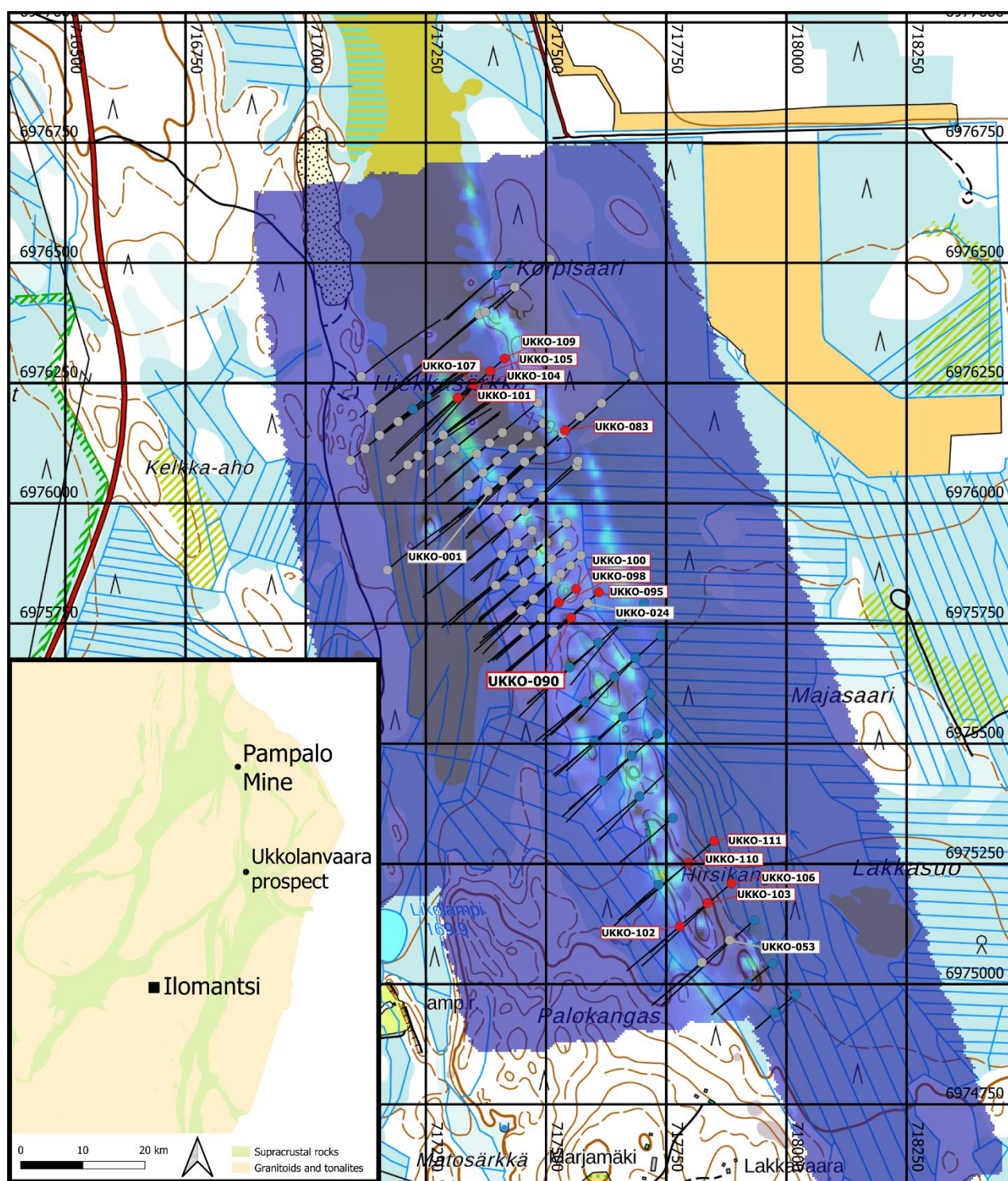
Figure 2 – Location map of the 2026 drill holes in Ukkolanvaara underlain by Total magnetic Intensity map
